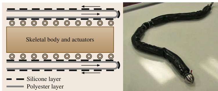
Fig. 20.9 The SAIC skin drive mechanism followed by the SAIC/CMU snake robot powered by the skin drive mechanism (after [20.25])
