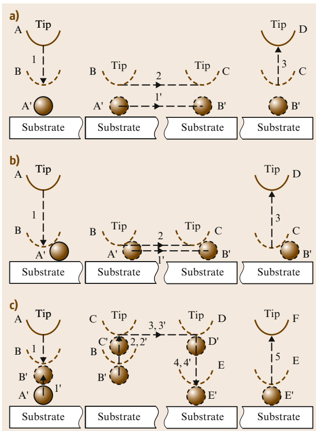
Fig. 27.15a–c Basic strategies of nanomanipulation. In the figure, A, B, C, ... represent the positions of end-effector (e.g., a tip); A', B', C', ... the positions of objects; 1, 2, 3, ... the motions of end-effector; and 1', 2', 3', ... the motions of objects. Tweezers can be used in pick-and-place to facilitate the picking-up, but are generally not necessarily helpful for placing. (a) Lateral noncontact nanomanipulation (sliding). (b) Lateral contact nanomanipulation (pushing/pulling). (c) Vertical nanomanipulation (picking and placing)
