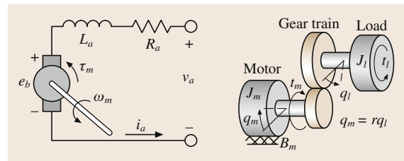
Fig. 4.17 Servomotor models
