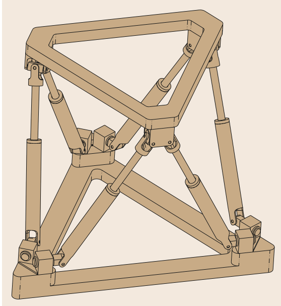
Fig. 18.1 Gough platform
