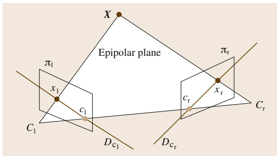
Fig. 34.7 A stereo vision system
