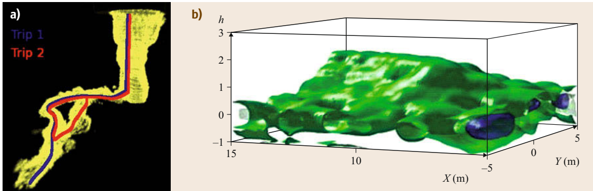
Fig. 45.13a,b Examples of volumetric maps for a natural environment. Whereas (a) shows a map of an underwater cave (after [45.23]), (b) depicts a terrain map obtained from a radar (after [45.24])
