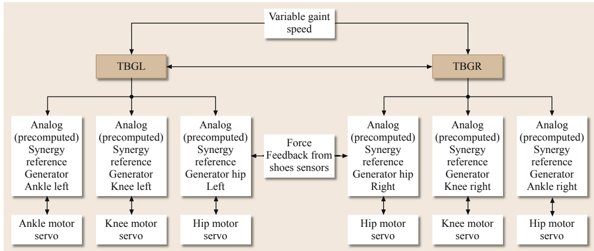
Fig. 70.17 The control structure of the 1974 Vokubratovic et al. 's exoskeletons (after [70.108]). The active device was powered with six pneumatic actuators whose references and feedback are determined through three different components: servo feedback, prescribed synergies, and force feedback for sagittal and lateral stabilization
