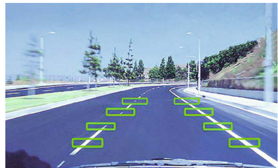
Fig. 62.8 Lane detection
