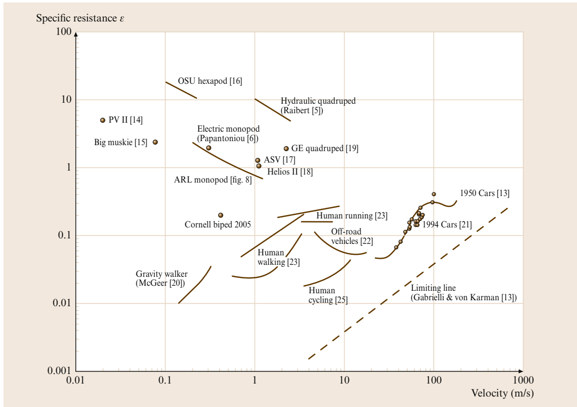
Fig. 17.39 Gabrielli-von Karman diagram (after [17.86])
