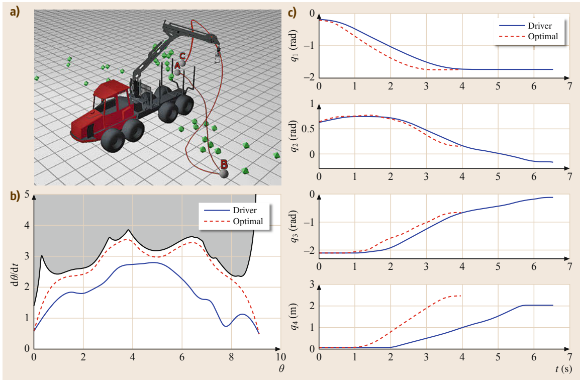
Fig. 56.27a–c Path-constrained replanning of human-operated motions. (a) Example of two crane motions performed by a human operator: from the load bunk to the logs (A–B) and back (B–C). (b) Velocity profiles for the distance \theta along the path A–B. A different distribution of the work between the joints allows for a higher velocity along the same path. The gray area indicates velocity constraints not to be violated. (c) The resulting evolution of joint coordinates with respect to time. The motion with a time-efficient velocity profile is clearly faster than the one of the driver
