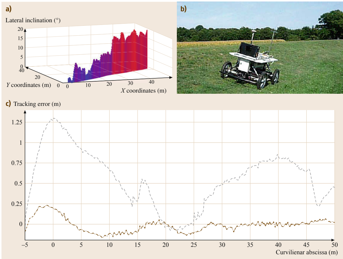
Fig. 49.19a–c Path following with sliding effects for an autonomous off-road robot: (a) Reference trajectory in 3-D frame (b) Robot during autonomous tracking (c) Tracking errors ( dashed : without sliding compensation, dash-dotted : with sliding estimation and compensation)
