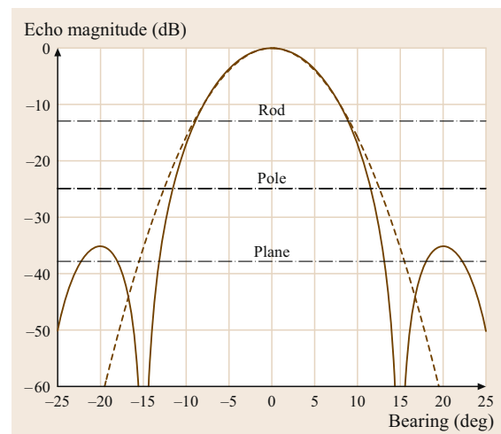
Fig. 30.11 Piston model transmitter/receiver pattern for the Polaroid 600 series transducer. A Gaussian approximation with SD = 5.25^\circ is shown in dashed line . Equivalent threshold levels for plane, pole, and rod objects at 1.5 m range are shown as dot-dashed lines
