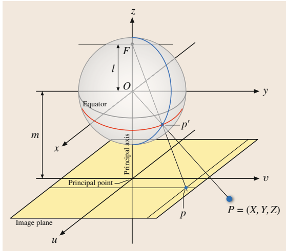
Fig. 34.8 Unified imaging model of Geyer and Daniilidis (after [34.7])
