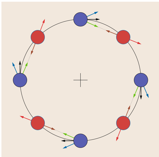
Fig. 34.5 Geometrical interpretation of IBVS: going from the blue position to the red one. In green, image motion when \mathbf{L}_e^+ is used in the control scheme; in blue, when \mathbf{L}_e^* is used; and in black when (\mathbf{L}_e/2 + \mathbf{L}_e^*/2)^+ is used (see the text for more details)
