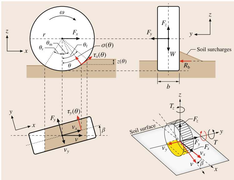
Fig. 50.8 Wheel–terrain contact model
