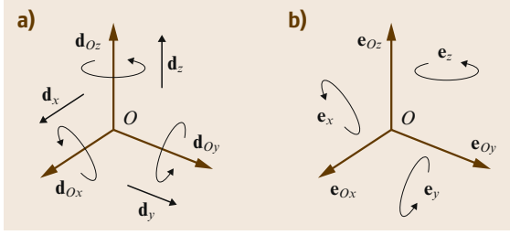
Fig.3.1a,b Plücker basis vectors for motions (a) and forces (b)
