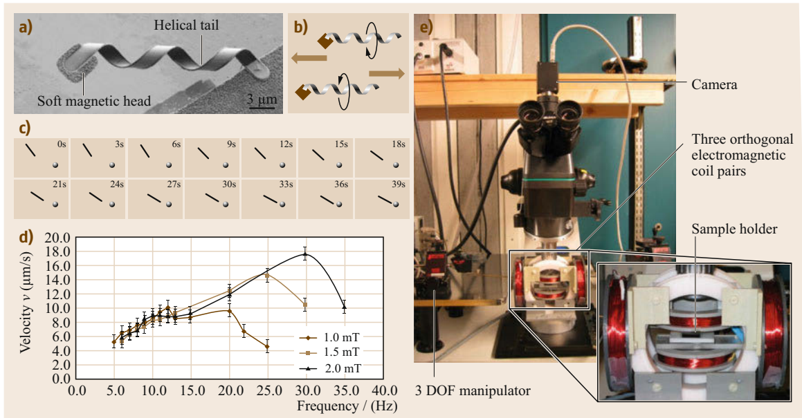
Fig. 27.12a–e Artificial bacteria flagella. (a) SEM micrograph of an as-fabricated ABF with a diameter of 2.7\ \mu\text{m} . (b) Schematic drawing of driving an ABF swims forward and backward as a rotary-to-linear motion converter. For forward and backward motion, the helical tail turns clockwise (CW) and counterclockwise (CCW), respectively (as seen by an observer in front of the ABF). (c) A series of frames taken from a video camera showing an ABF swim forward in water. The ABF has an 81\ \mu\text{m} long InGaAs/GaAs/Cr helical tail, and a 4.5\ \mu\text{m} \times 4.5\ \mu\text{m} square head. B, f, \theta, \varphi represent four parameters, i. e., magnetic field, field frequency, yaw and pitch, which can be controlled by the coil pairs. (d) The dependence of ABF velocity to frequency of external magnetic field generated by the coil pairs. (e) Experimental setup. All examples are from the authors' work
