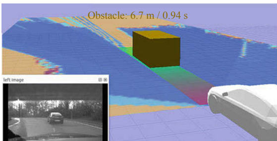
Fig. 62.9 Instantaneous representation of the navigable space in front of the vehicle (after [62.25])
