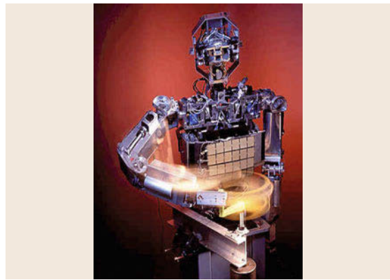
Fig. 67.10 The humanoid robot Cog used neural oscillators in conjunction with compliant torque-controlled arms to perform a variety of everyday tasks with human tools, such as crank turning, hammering, sawing, and playing a snare drum (after [67.32]; courtesy Sam Ogden)
