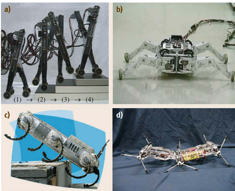
Fig.17.33a–d Leg-wheel hybrid robots. (a) Biped leg–wheel robot (1998); (b) Roller walker (1996); (c) RHex (2001); (d) Whegs II (2003) (after [17.65–68])
