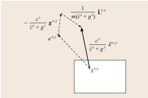
Fig. 48.3 The horizontal acceleration \ddot{c}^{x,y} of the COM of the robot is the sum of a force pushing the COM c^{x,y} away from the CoP z^{x,y} the effect of gravity -\mathbf{g}^{x,y} and variations \dot{\mathbf{L}}^{x,y} of the angular momentum
