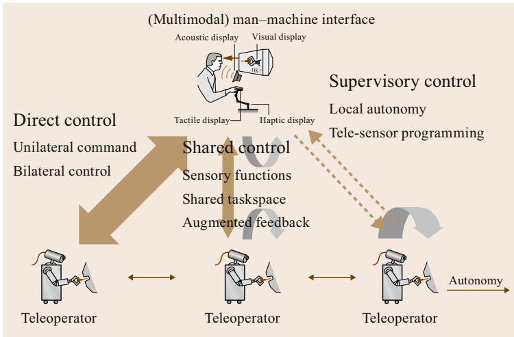
Fig. 43.10 Different concepts for telerobotic control architectures
