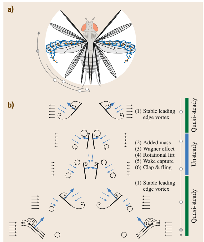
Fig.26.31a,b Flapping insect wing aerodynamics can be understood through the interaction of a myriad of complex aerodynamic mechanisms. (a) The key high-lift mechanism insects employ, is a stable leading edge vortex (LEV) generated during the up and downstroke. (b) A flapping cycle consists of a quasi-steady part during which the wing accelerates little. During this phase, the stable LEV is the key high-lift mechanism (1). During stroke reversal there is evidence that up to five effects (2)–(6) could be important (after [26.44])
