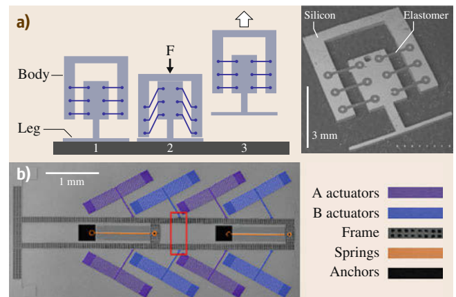
Fig. 23.21 (a) Microrobot (after [23.101]), (b) a colored SEM image of the actuated mechanism (after [23.101])
