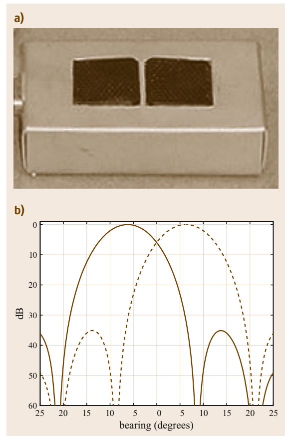
Fig. 30.30a,b Binaural vergence sonar (a) and beam patterns (b) along the sonar axis with vergence angle \alpha = 8^\circ : solid-left transducer, dashed-right transducer
