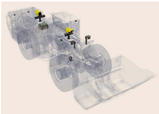
Fig. 59.15 Scooptram (or LHD) components for robotic tramping, including SICK scanning laser rangefinders (front and rear), articulation angle encoder, drive shaft encoder, onboard cameras, and computing subsystems (courtesy of Atlas Copco, 2009)
