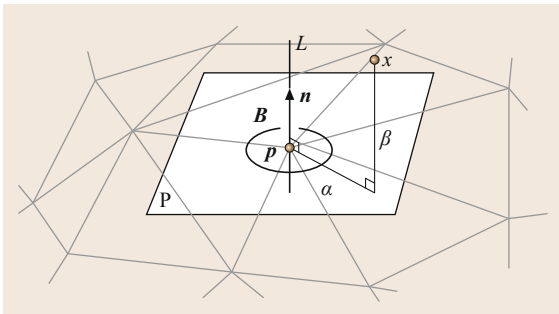
Fig. 31.13 Definition of a spin image
