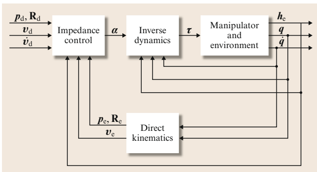
Fig. 9.1 Impedance control
