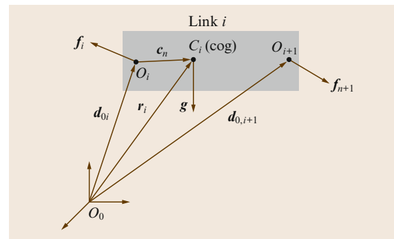
Fig. 6.11 Dynamics of the last link
