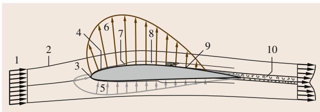
Fig. 26.7 Characteristics of a 2-D flow around an airfoil 1 – Free stream velocity field, 2 – Streamline, 3 – Stagnation point, 4 – y-Laminar boundary layer, 5 – Overpressure, 6 – ySuction, 7 – Transition point, 8 – Turbulent boundary layer, 9 – Separation point, 10 – Separated flow
