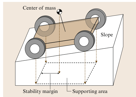
Fig. 58.23 Stability condition
