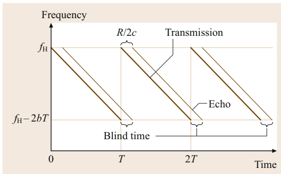
Fig. 30.21 Plot of frequency versus time for CTFM. The blind time applies if the shown echo corresponds to a maximum range target at R_m
