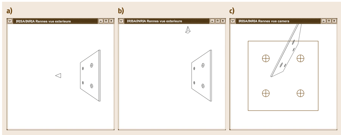
Fig.34.1a–c Example of positioning task: (a) the desired camera pose with respect to a simple target, (b) the initial camera pose, and (c) the corresponding initial and desired image of the target
