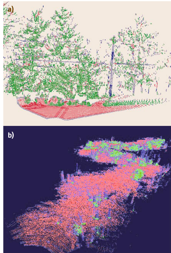
Fig.45.12a,b Example of mapping and classification of 3-D point sets: (a) 3-D data and classification result ( green = vegetation, red = surfaces, blue = lines; the saturation of the color is proportional to the confidence in the classification result); (b) map accumulated over a large number of scans
