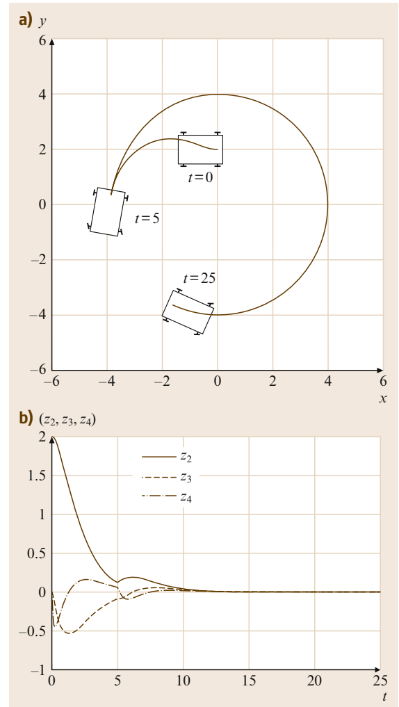
Fig. 49.9a,b Path following along a circle. (a) Cartesian motion; (b) coordinates z_{2,3,4} versus time
