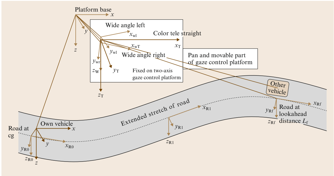
Fig. 35.6 EMS-Vision road scene tree
