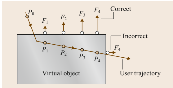
Fig. 42.8 Illustration of subtle aspects of haptic rendering of contact force. The operator fingertip trajectory enters object surface moving down and to right. Haptic interaction points (HIP) are shown at times 1–4 (solid circles, P_0 – P_4 ). Intermediate haptic interaction points (IHIP) are shown when the HIP is inside the object (open circles). At position P_4 , the algorithm must not render force based on the closest surface point or the operator will be ejected from the side of the object (feeling unnatural force tangential to the top surface)
