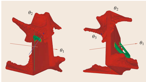
Fig. 36.14 Two views of the set of goal configurations (green) for grasping a cylindrical part in a disconnected C-space
