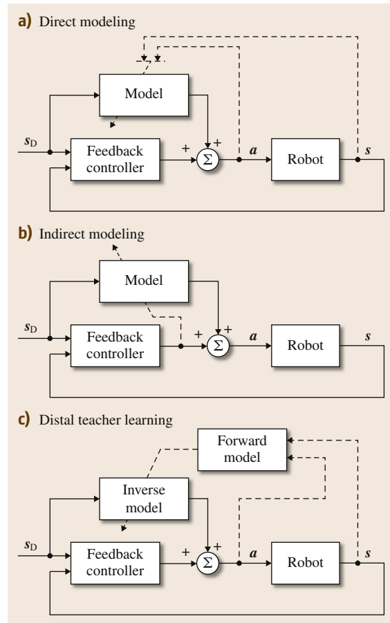
Fig. 15.3a–c Learning architectures in model learning applied to control. (a) In the direct modeling approach, the model is learned directly from the observations – the given example shows learning and inverse model. (b) Indirect modeling approximates the model using the output of the feedback controller as error signal. (c) In the distal teacher learning approach, the inverse model’s error is determined using the forward model. The resulting models will converge to an identity transformation
