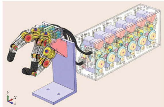
Fig. 4.5 The Salisbury three-fingered robot hand with its cable drive system
