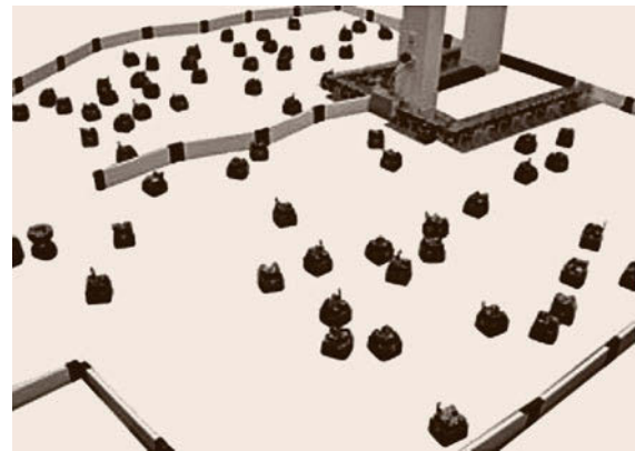
Fig. 53.12 The SwarmBot robots
