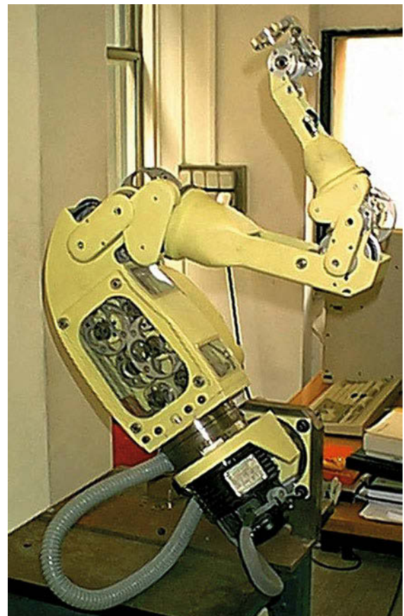
Fig. 11.2 The cable-driven robot Dexter by Scienza Machinale
