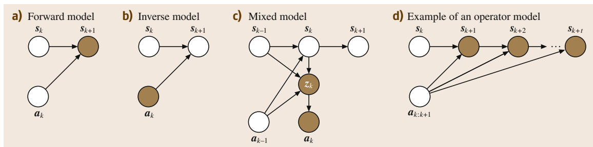
Fig.15.2a–d Graphical models for different types of models. The white nodes denote the observed quantities, while the brown nodes represent the quantities to be inferred . (a) The forward model allows inferring the next state given current state and action. (b) The inverse model determines the action required to move the system from the current state to the next state. (c) The mixed model approach combines forward and inverse models in problems where a unique inverse does not exist. Here, the forward and inverse models are linked by a latent variable z_k . (d) The operator model is needed when dealing with finite sequences of future states
