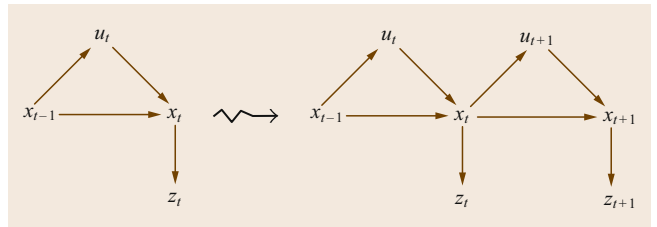
Fig. 14.2 Unfolding of a simple DBN over two time slices representing two successive states. Variables x denote states, u denote actions, and z denote measurements. The structure of each individual slice (signaled by identical variable subscripts) is invariant over time
