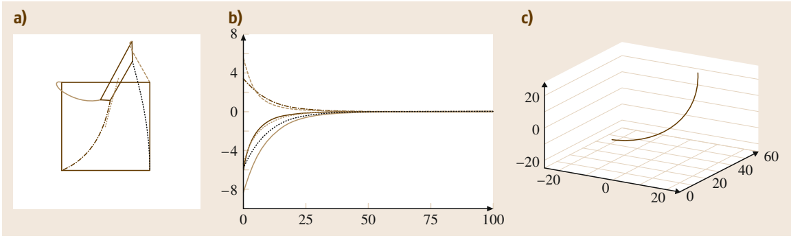
Fig. 34.12 2.5-D VS system behavior using s = (\mathbf{x}_g, \log(Z_g), \theta \mathbf{u}) (refer to Fig. 34.2a-c for description)
