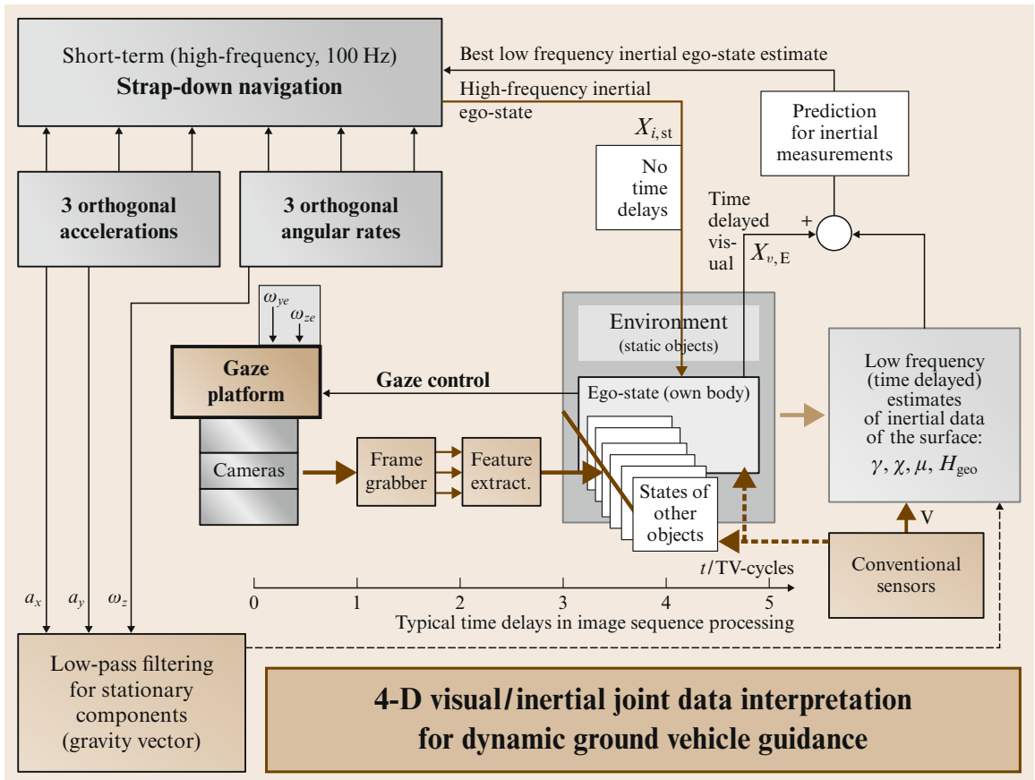
Fig. 35.7 EMS-Vision guidance system
