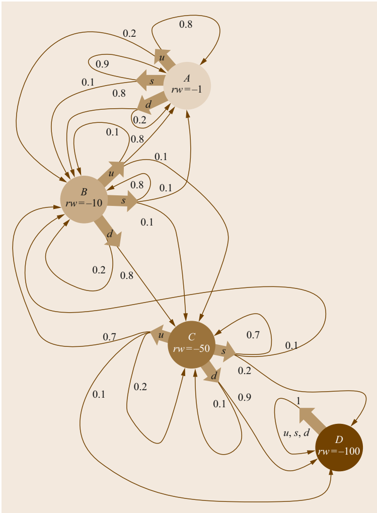
Fig. 14.4 A representation of an MDP. In this example, states A , B , C , D have associated rewards (−1, −10, −50, −100). There are three possible actions in each state, u , s , d , each have a given probability (shown on the arrows) to lead to another state
