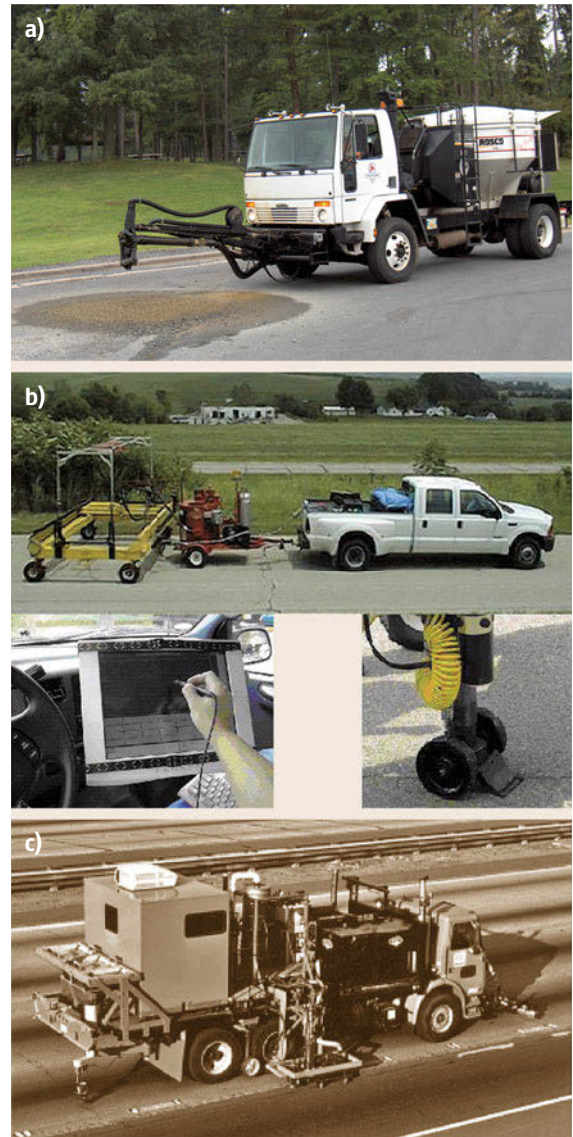
Fig.57.26a–c Road maintenance: (a) Teleoperated pothole patching robot (courtesy Leeboy); (b) semi-autonomous road crack sealing robot (after [57.57]); (c) semi-autonomous road crack sealing robot (after [57.58])
