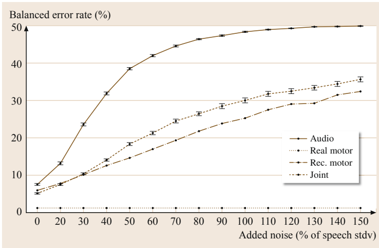
Fig. 77.11 Comparison of acoustic versus motor features under increasing level of added Gaussian white noise for the same classifier of the previous experiments
