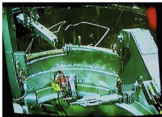
Fig. 58.16 Operator's view of a remote sawing task (courtesy of Oak Ridge National Laboratory)
