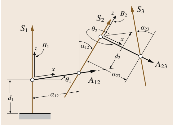
Fig. 4.8 The kinematic skeleton defined by the joint axes and their common normals
