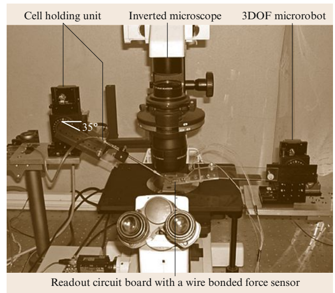
Fig. 27.9 Robotic biomanipulation system with vision and force feedback
