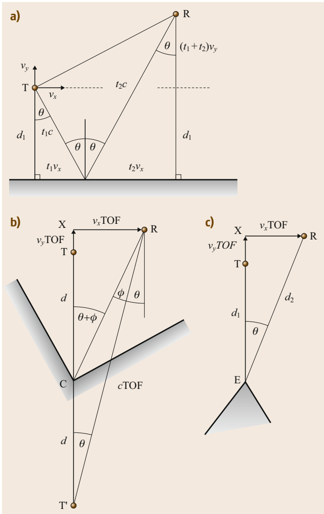
Fig.30.27a–c Observing a target from a moving sensor. T is the position of the transmitter and R is where the echo is received at the end of the TOF. The target is a plane in (a), a corner in (b), and an edge in (c)
