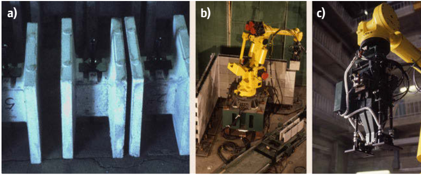
Fig. 57.4 (a) Building component developed by guidelines of Robot Oriented Design (ROD), (b) SMAS total system, (c) robot end-effector/gripper with optical fiber sensor guiding screwing mechanism
