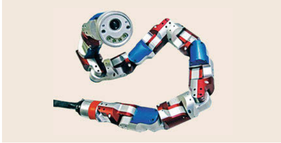
Fig. 20.6 Choset's Modsnake consisting of 16 DOFs (degree of freedom) each orthogonally placed with respect to each other (after [20.17, 18])
