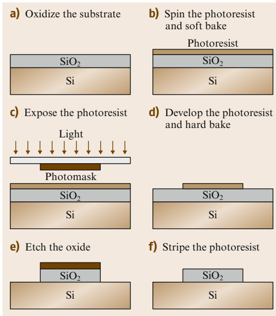
Fig.27.3a–f Schematic drawing of the photolithographic steps with a positive photoresist (PR) (a) Oxidize the substrate (b) spin the photoresist and soft bake (c) expose the photoresist (d) develop the photoresist and hard bake (e) etch the oxide (f) stripe the photoresist
