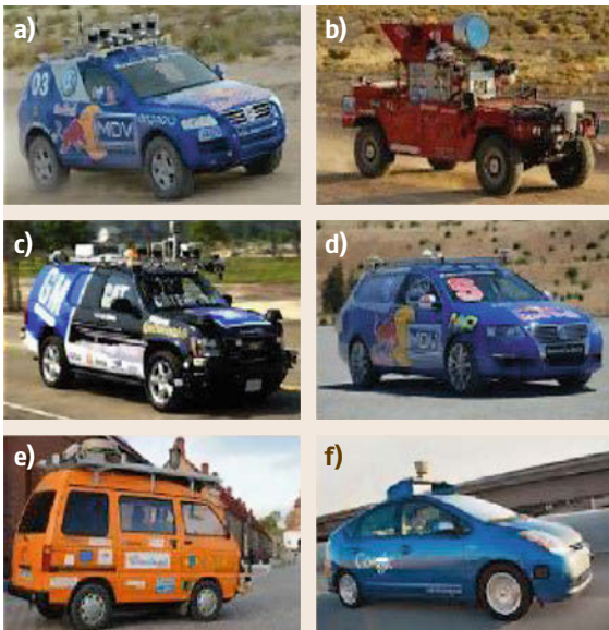
Fig. 62.3a–f 2005 Grand Challenge vehicles: (a) Stanley (1st), (b) Sandstorm (2nd), 2007 Urban Challenge vehicles, (c) Boss (1st), (d) Junior (2nd), (e) VisLab and (f) Google vehicles
