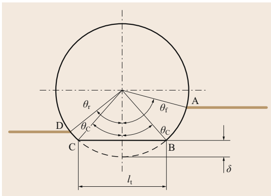
Fig. 24.13 Diagram of deformable wheel traveling over deformable terrain
