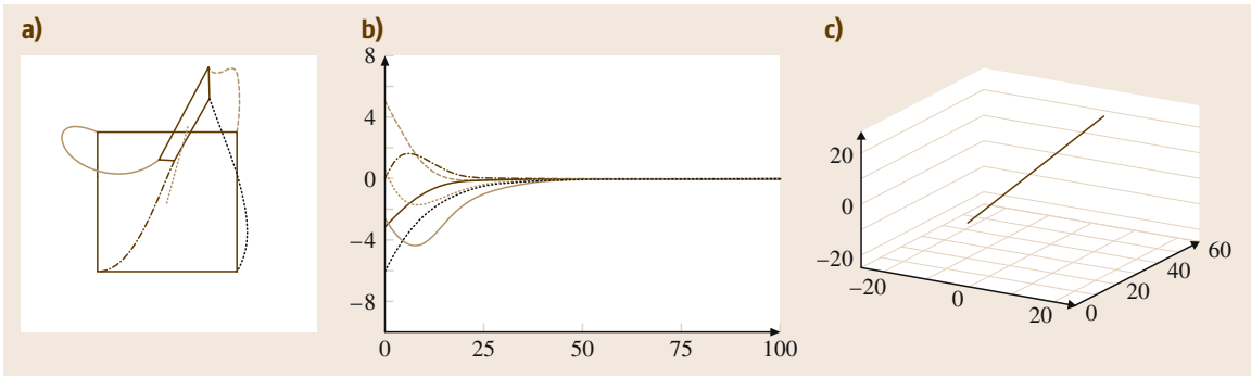
Fig. 34.13 2.5-D VS system behavior using s = (c^* \mathbf{t}_c, \mathbf{x}_g, \theta \mathbf{u}_z) (refer to Fig. 34.2a-c for description)
