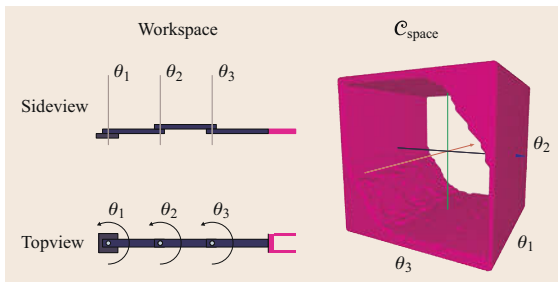
Fig. 36.9 Non-planar 3 DOF manipulator and corresponding self-collision C -obstacle
