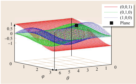
Fig. 31.16 Transformation of three points from \mathbb{R}^3 to the Hough space (\theta, \varphi, \rho) . The intersection of the curves (marked in black) depicts the plane spanned by the three points
