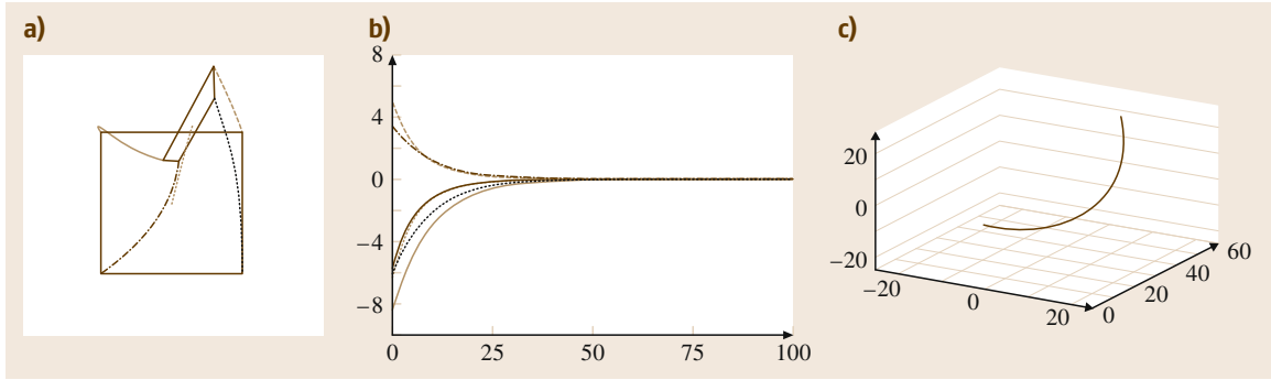
Fig. 34.9 PBVS system behavior using s = ({}^c t_o, \theta u) (refer to Fig. 34.2a-c for description)
