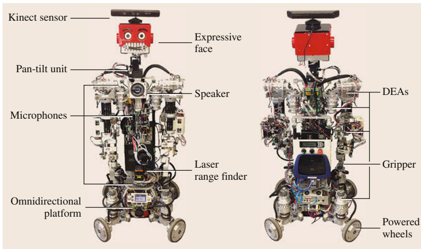
Fig. 13.5 Photographs of the front and back of the robot, IRL-1 (30 DOF and 55 sensors). DEAs stand for Differential Elastic Actuators (after [13.133])
